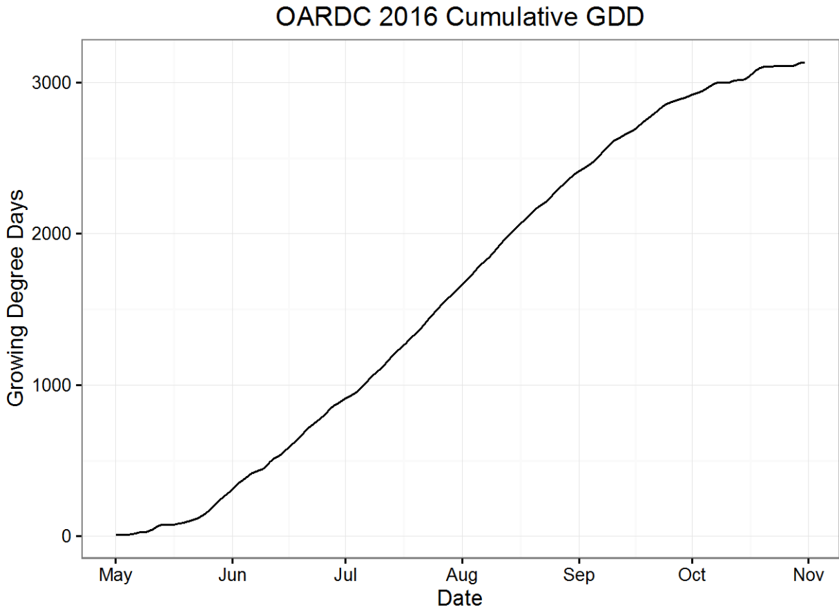
Figure 2. 2016 Cumulative Growing Degree Days at OARDC from May – November.
