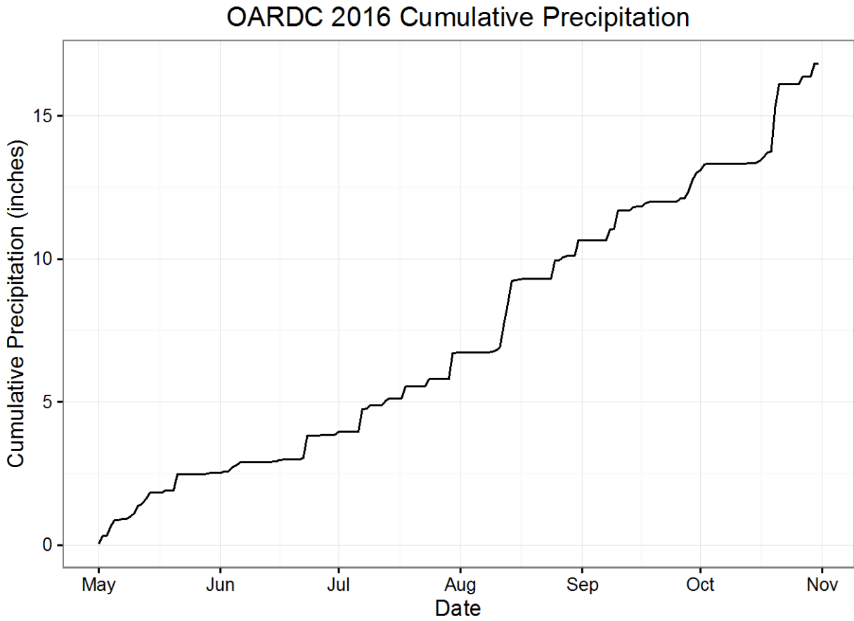
Figure 1. 2016 Cumulative Precipitation at OARDC from May – November.
